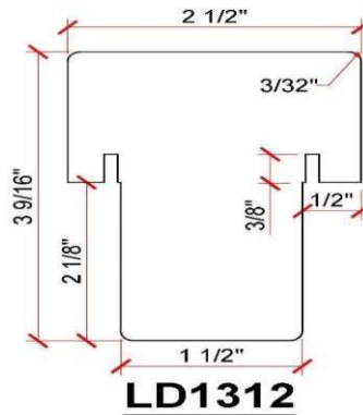
LD1312 Mull Post (LD1312-N: NAFS)
