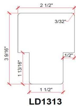
LD1313 Mull Post
