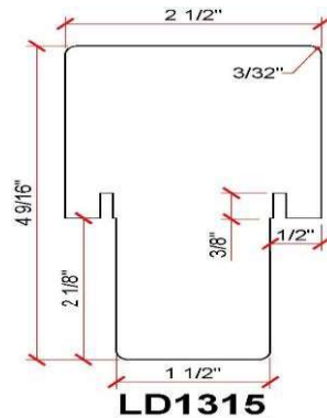
LD1315 Mull Post (LD1315-N: NAFS)
