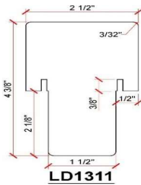
LD1311 Mull Posts (LD1311-N: NAFS)
